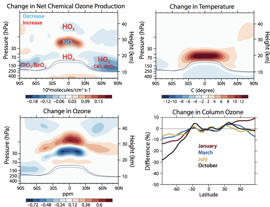
FIGURE 2.3 Processes impacting stratospheric ozone in 2042–2049 following RCP8.5 for 16 Tg S yr -1 injections at 15°N/15°S. Impact of enhanced sulfate aerosols on zonal and annual averaged net rate of chemical production of ozone (top left), temperature (top right), and ozone concentration (bottom left). Changes in the dominant ozone loss cycles are shown in blue if decreasing (net chemical production is increasing) and in red if increasing (net chemical production decreasing) (top left). Differences in column ozone (%) between the geoengineering and the control simulation in 2042–2049 are illustrated for different months (bottom right). SOURCE: WMO (2018).
