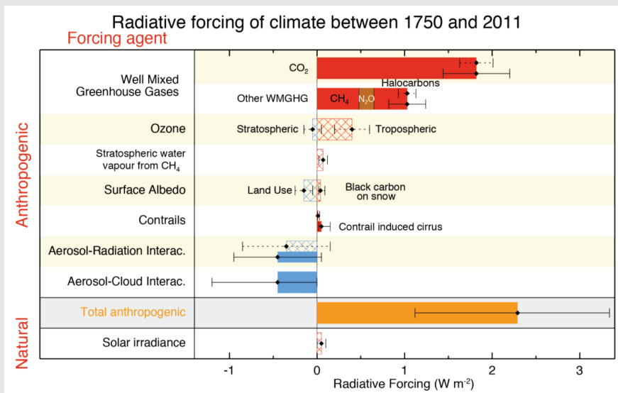
FIGURE 2.2.1 Global, annual mean radiative forcings ( \text{W m}^{-2} ) due to key climate forcing agents, for the period from pre-industrial to 2011. Note that some of these effects remain poorly understood and even the sign of forcing (positive/negative) is uncertain. SOURCE: IPCC (2018).
